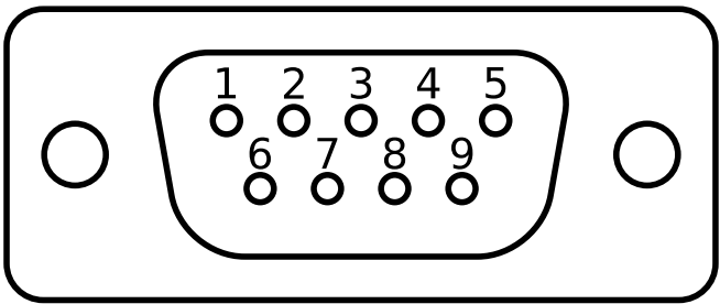
Illustration 2: DB9 connector pin-out for OBDII Odometer
